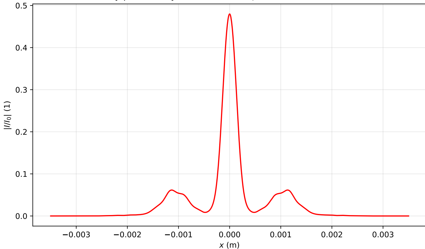
Intensity profile I(x, y = 0, z = 2.627)/I_0 , P_{in}=8.5P_{cr} , artificial time
